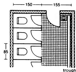
⑥ Doors opening inwards; with urinal trough
